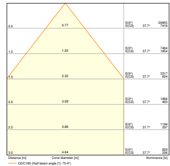
HB P 75W 865 110DEG IP66 PS - REFRACTOR
